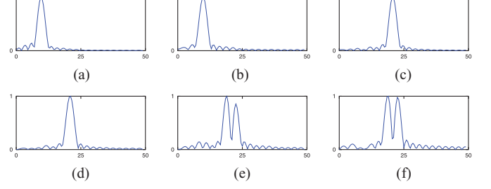
Fig. 5. Amplitude characteristics of the filters designed by DFBCSP1 with in subject ay . (a) First filter. (b) Second filter. (c) Third filter. (d) Fourth filter. (e) Fifth filter. (f) Sixth filter.
