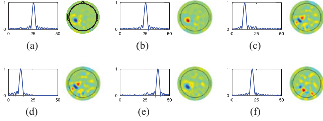
Fig. 4. Filters and the associated spatial weights designed by DFBCSP1 in subject aa . (a) First filter. (b) Second filter. (c) Third filter. (d) Fourth filter. (e) Fifth filter. (f) Sixth filter.
