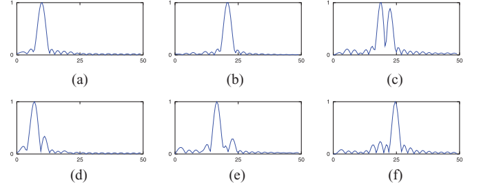
Fig. 6. Amplitude characteristics of the filters designed by DFBCSP2 with in subject ay . (a) First filter. (b) Second filter. (c) Third filter. (d) Fourth filter. (e) Fifth filter. (f) Sixth filter.
